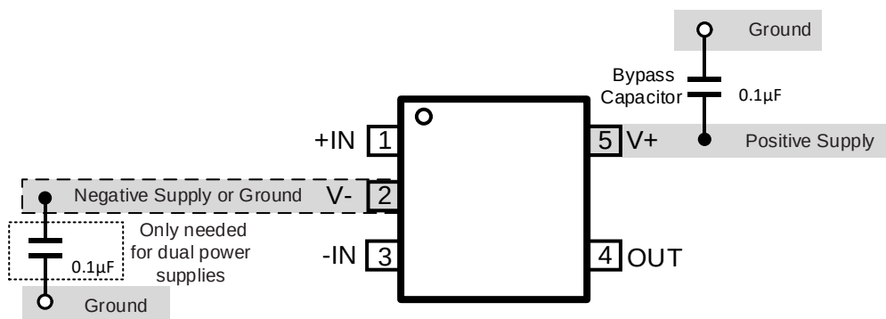
Figure 4. LM331 Layout Example
